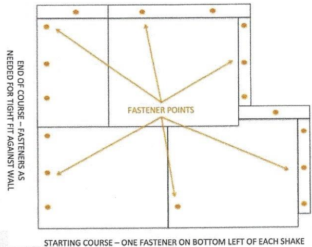
FIGURE 3 – VAPORLOCK INSTALL FRONT VIEW
